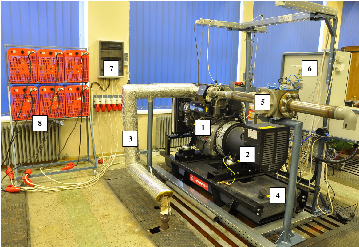
Fig. 1. Experimental setup
